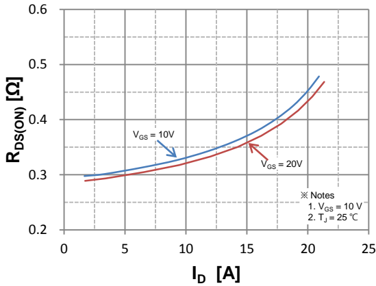
R DS(on) [Ω] Figure 3. On Resistance Variation vs Drain Current and Gate Voltage
