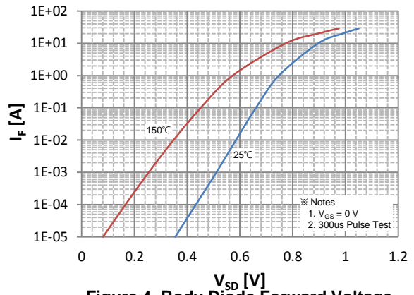
I F [A] V SD [V] Figure 4. Body Diode Forward Voltage Variation with Source Current and Temperature
