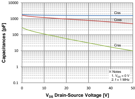
Figure 3. Capacitance Characteristics
