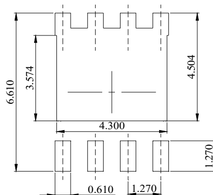
DIMENSIONS: MILLIMETERS
