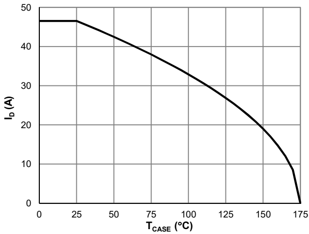
Figure 7: Current De-rating
