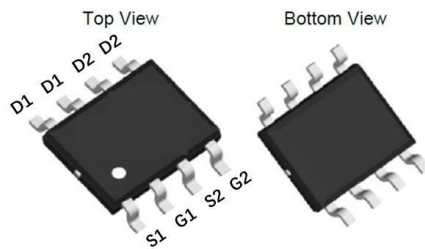
SOP-8(Dual)
